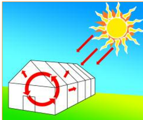
Figure 5. The heat-trapping ability of a greenhouse is influenced by a number of factors, including the transparency of the greenhouse cover, and colour and type of surfaces of the greenhouse.
