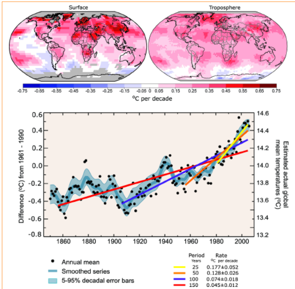
Figure 9. (Top) Patterns of linear global temperature trends over the period 1979 to 2005 estimated at the surface (left), and for the troposphere from satellite records (right). Grey indicates areas with incomplete data.
