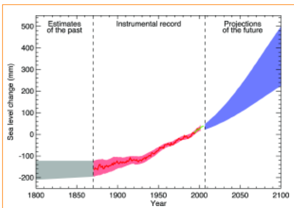
Figure 10. Time series of global mean sea level (deviation from the 1980-1999 mean) in the past and as projected for the future. For the period before 1870, global measurements of sea level are not available. The grey shading shows the uncertainty in the estimated long-term rate of sea level change. The red line is a reconstruction of global mean sea level from tide gauges and the red shading denotes the range of variations from a smooth curve. The green line shows global mean sea level observed from satellite altimetry. The blue shading represents the range of model projections of the Special Report on Emissions Scenarios (project A1B) for the 21st century, relative to the 1980 to 1999 mean, and has been calculated independently from the observations. Beyond 2100, the projections are increasingly dependent on the emissions scenario. Over many centuries or millennia, sea level could rise by several metres. (Source: IPCC, 2007b, p.111).
