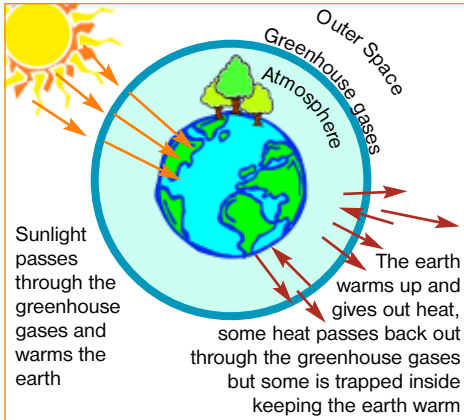
Figure 6. Greenhouse effect Source: Impetus Consulting Ltd.
