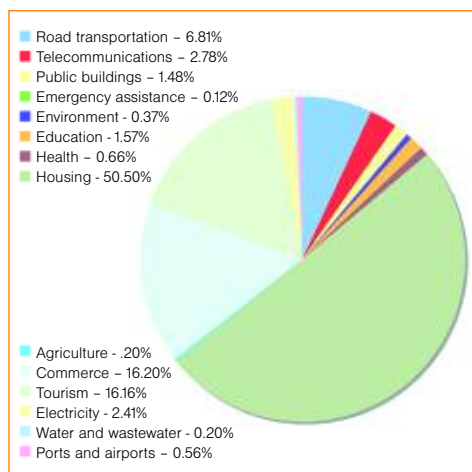
Figure 11. Breakdown of damage and losses in the Cayman Islands, Hurricane Ivan 2004 Source: Zapata Marti, 2005
