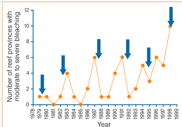
Figure 3. Number of reef provinces bleaching since 1978. Arrows indicate strong El Niño years. While some of the trend can be explained by observer bias, this factor does not completely explain the increasing trend with time. Source: Hoegh-Guldberg 1999
