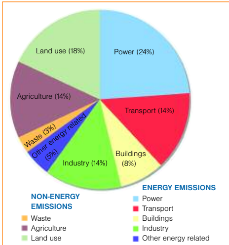
Figure 7. Greenhouse-gas emissions in 2000, by source. Source: Prepared by Stern Review, from data drawn from World Resources Institute Climate Analysis Indicators Tool (CAIT) on-line database version 3.0.
