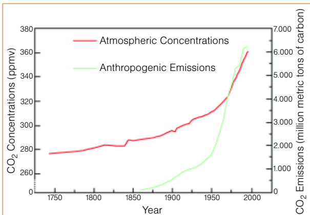
Figure 8. Trends in Atmospheric Concentrations and Anthropogenic Emissions of Carbon Dioxide Source: Oak Ridge National Laboratory.
