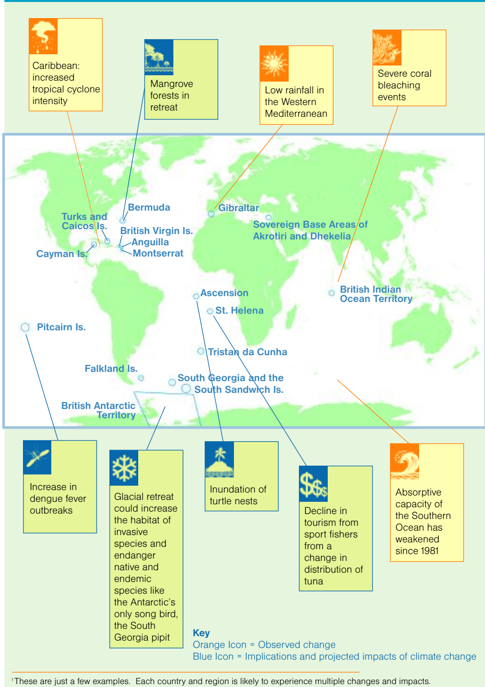
Figure 1. Selected global warming changes and impacts in UK Overseas Territories 1
