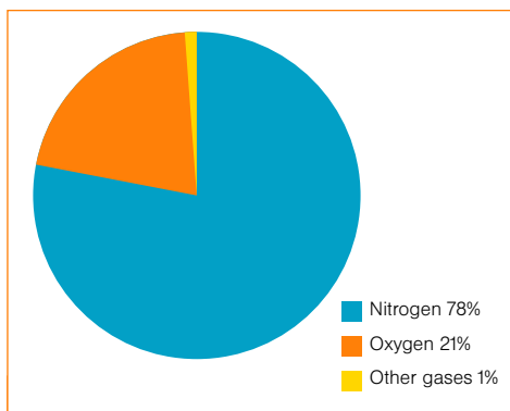
Figure 4. Gases in the atmosphere
